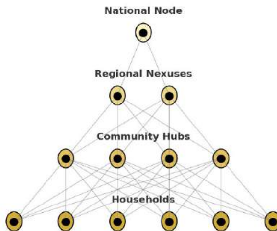
Pyramid-to-Network: From Households to National Nodes
